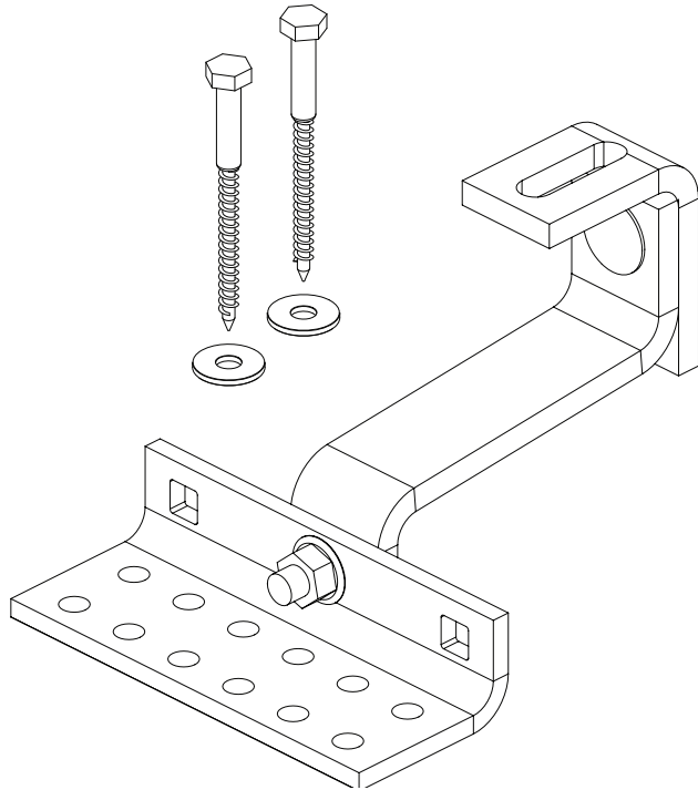
Exploded View (lag screws not included)
