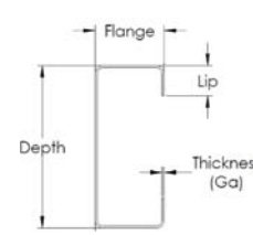
TYPICAL PROFILES
