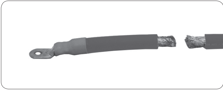
Fig. 3.18. Battery end of Positive cable cut and prepared for inserting into the Class "T" Fuse Assembly
